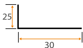
Cantoneira Lisa 25 x 30
